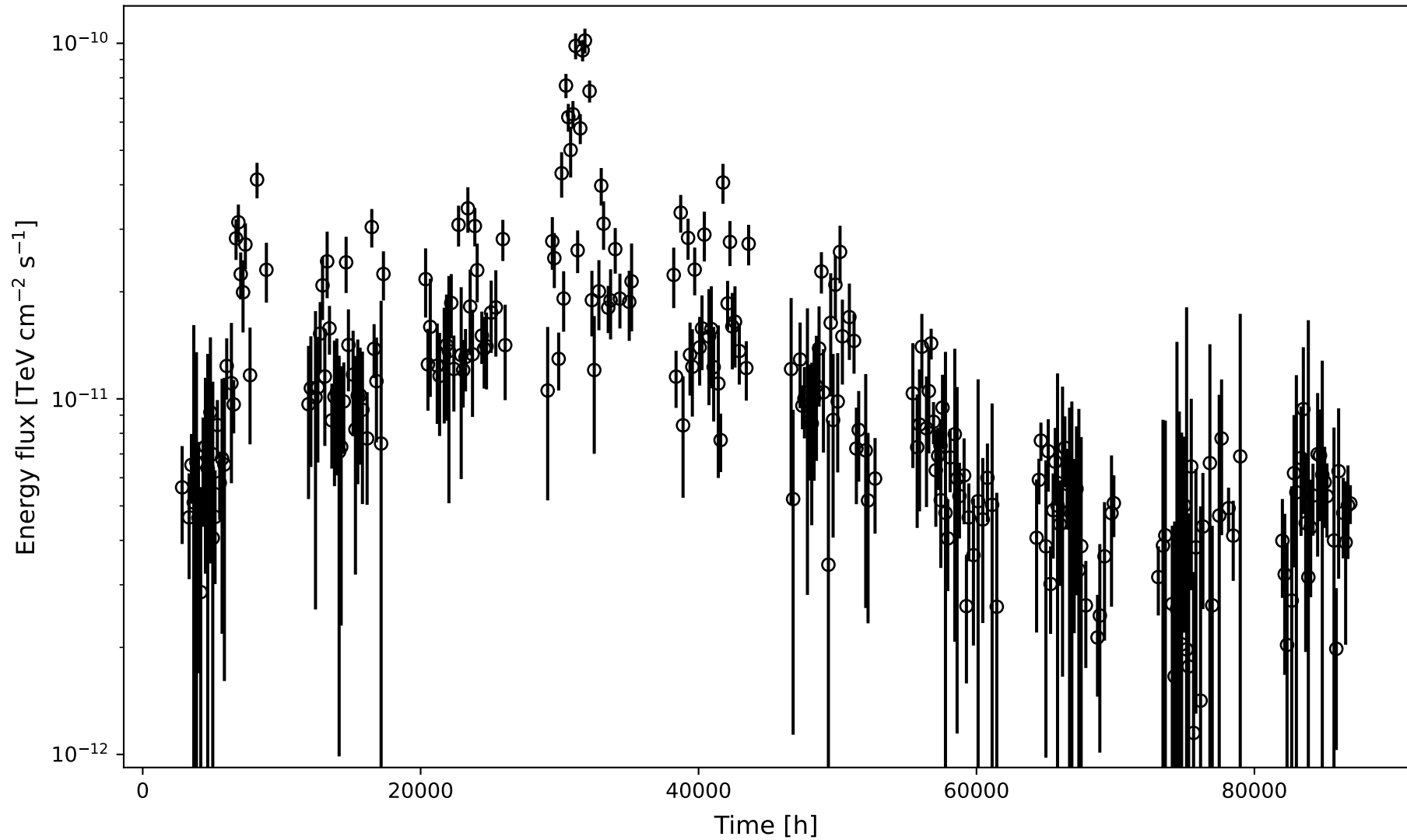
BLLac, cadence - 30 min 1 time per week - CTAO simulation
